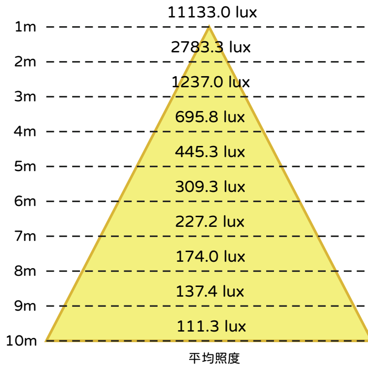
3200 60° Illuminance diagram
